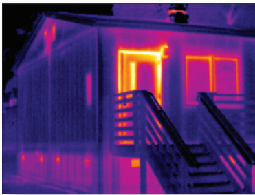
Full infrared
